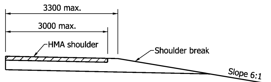
SECTION F-F
