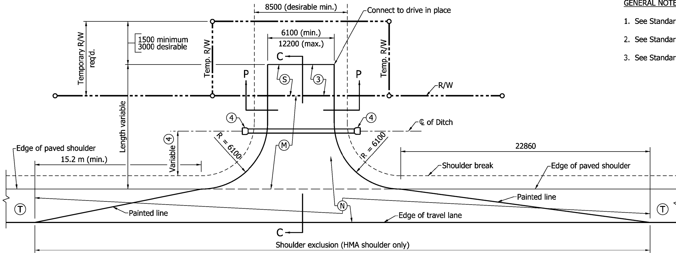
PLAN VIEW (PAVED SHOULDER 2400 OR GREATER IN WIDTH)
