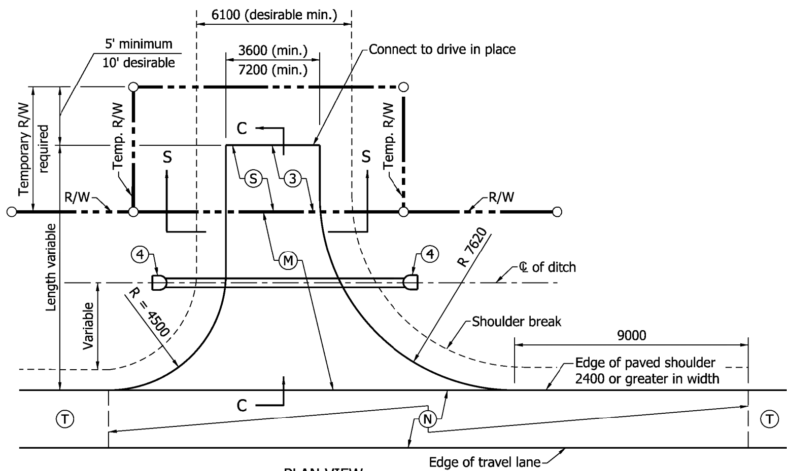
PLAN VIEW (PAVED SHOULDER 2400 OR GREATER IN WIDTH)
