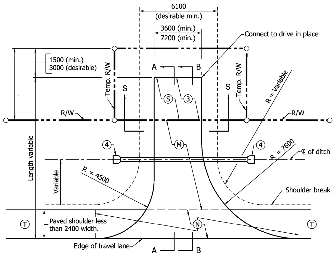
PLAN VIEW (PAVED SHOULDER LESS THAN 2400 IN WIDTH OR UNPAVED SHOULDER)
