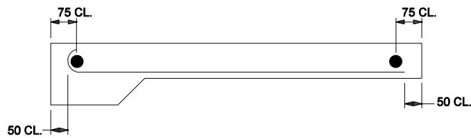
X - SECTION THROUGH APPROACH (One Layer of Steel Shown)
