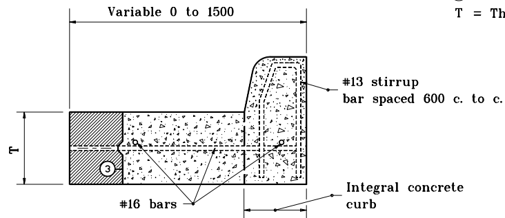
SECTION C-C
