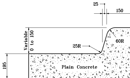
MONOLITHIC CURB
