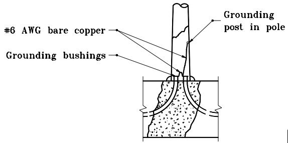
BRIDGE GROUNDING
