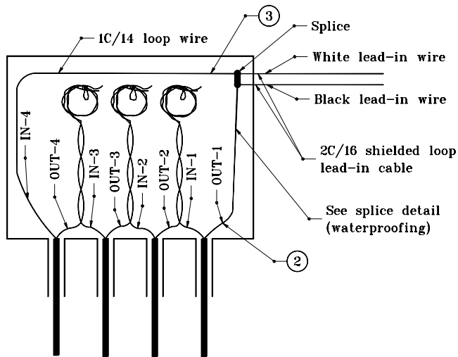
① DETAIL A DETECTOR HOUSING WIRING
