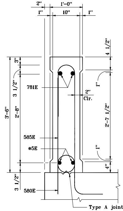
SECTION B-B
