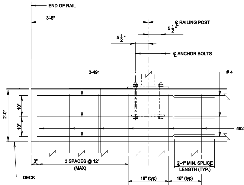
ELEVATION VIEW
