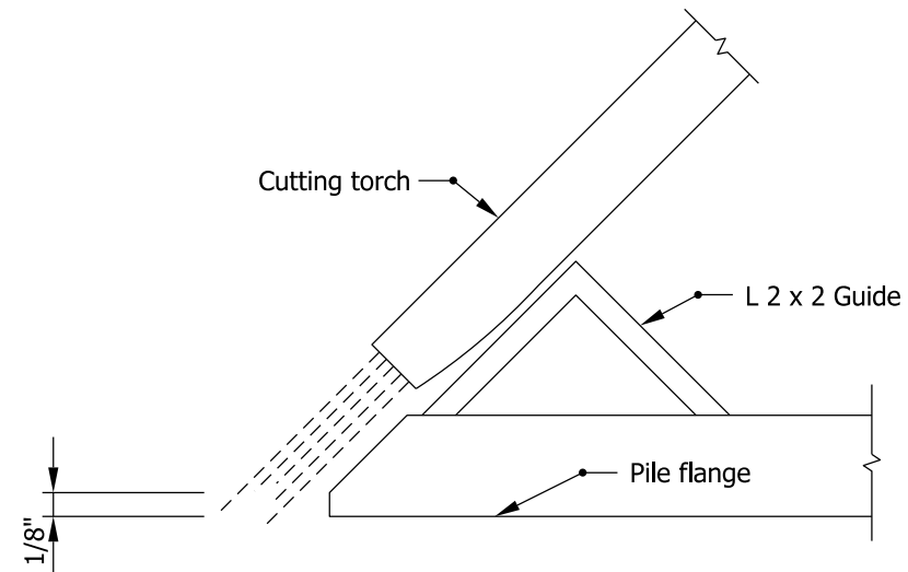
SUGGESTED METHOD TO BEVEL FLANGE
