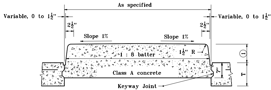
SECTION K-K
