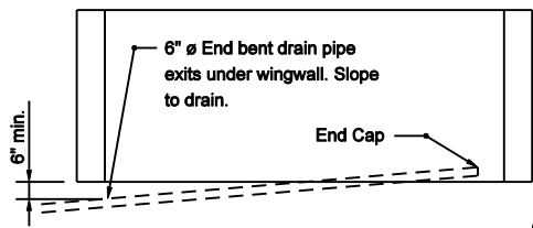
ELEVATION - END BENT
