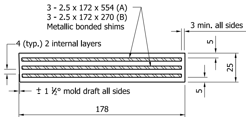
SECTION E-E TYPE 7
