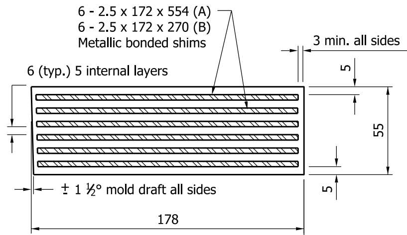
SECTION E-E TYPE 5
