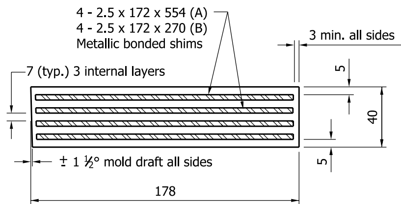
SECTION E-E TYPE 6
