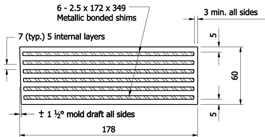
SECTION A-A TYPE 1
