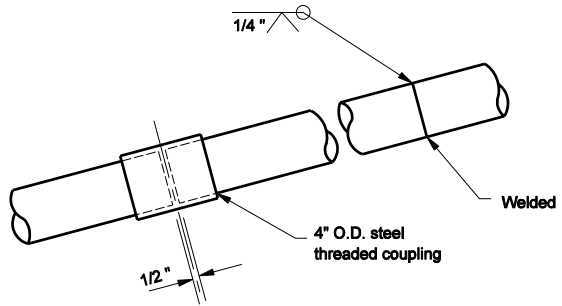
OPYIONAL COUPLING
