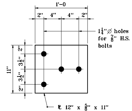
PLATE WASHER PWW
