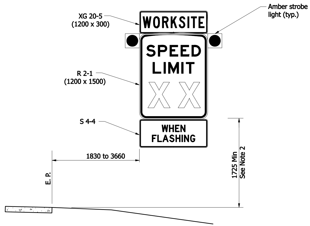
Worksite Speed Limit Sign Assembly
