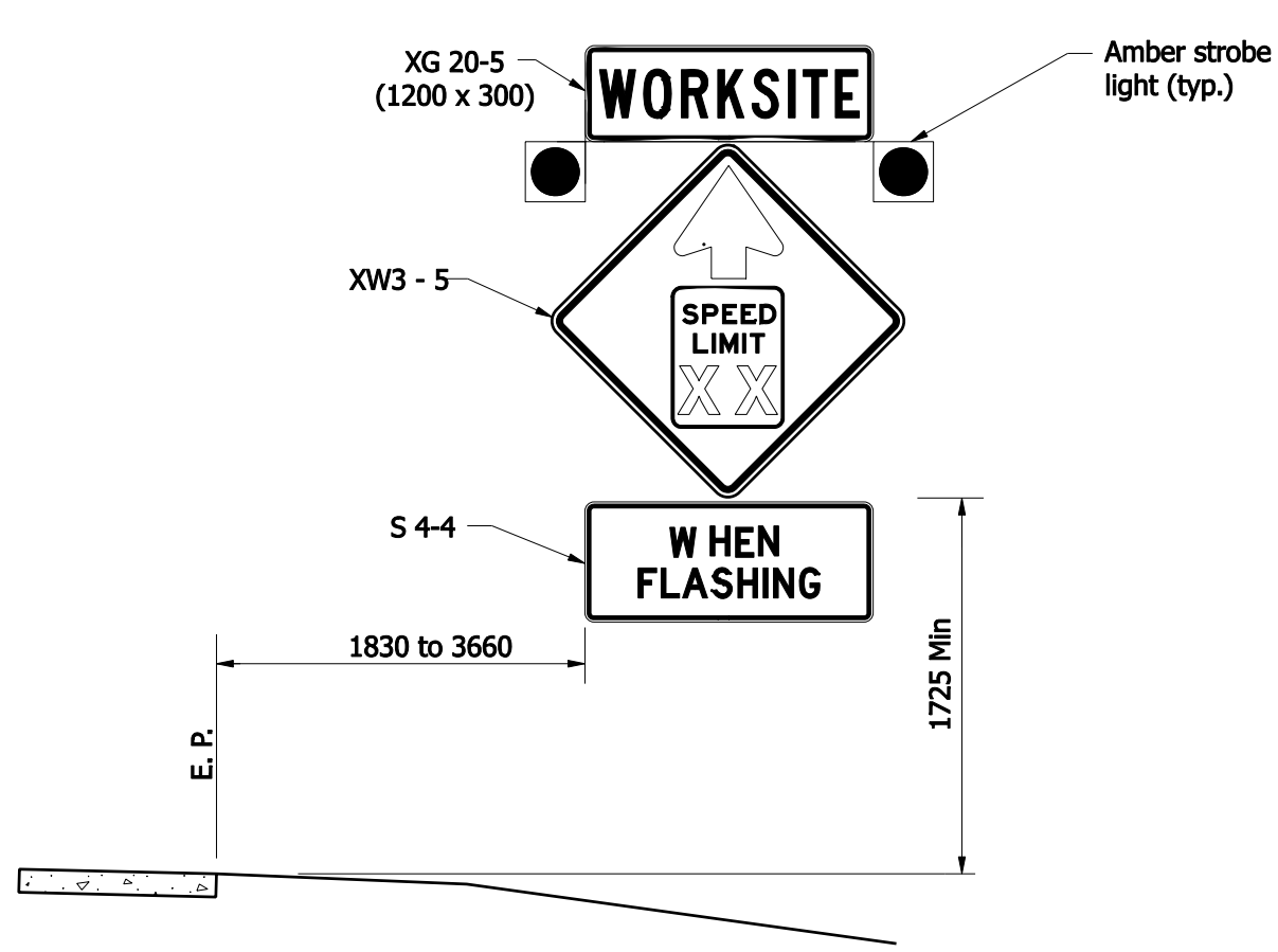
Reduced Speed Advance Warning Sign Assembly
