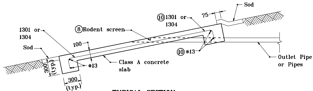
TYPICAL SECTION
