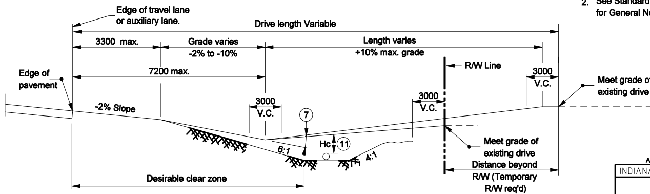
TYPICAL PROFILE GRADE IN CUT
