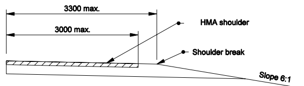
SECTION F-F
