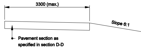
SECTION E-E
