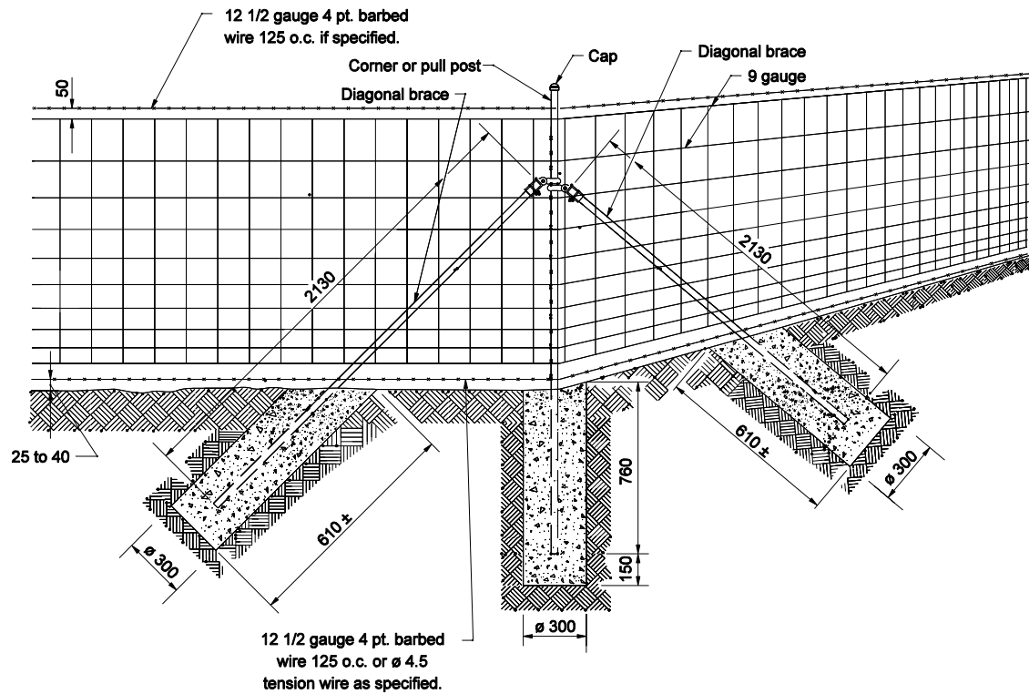
FARM FIELD TYPE FENCE CORNER
