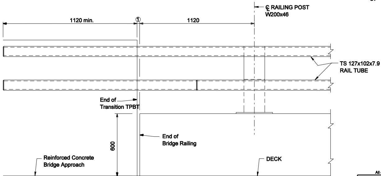
RAILING ELEVATION AT ENDS
