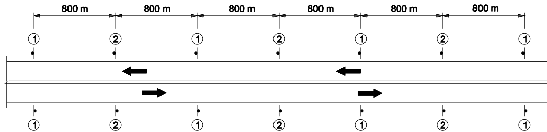
CONSTRUCTION SIGNS LOCATION DETAIL
