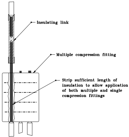
DETAIL D
