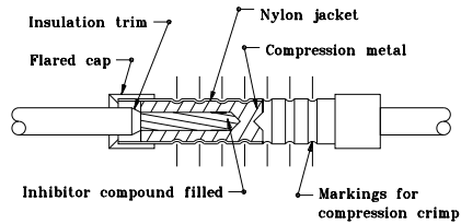
DETAIL C INSULATING LINK
