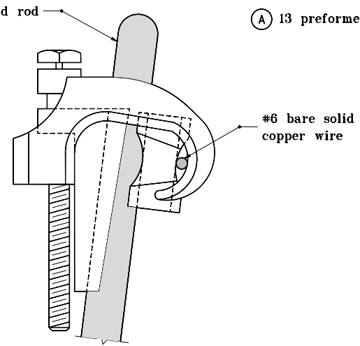
GROUNDING GRID
