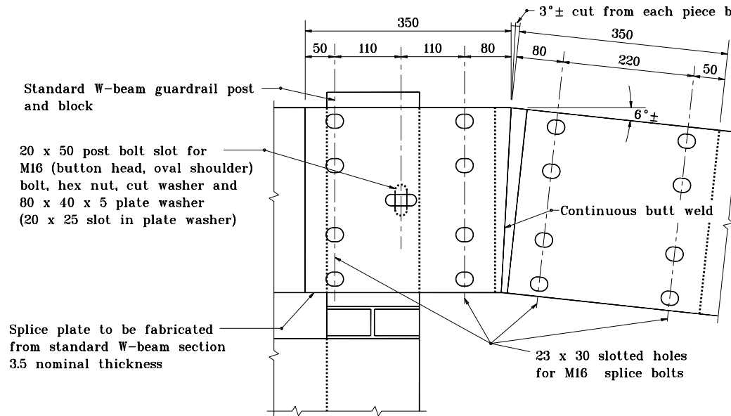
SPLICE PLATE ASSEMBLY DETAIL
