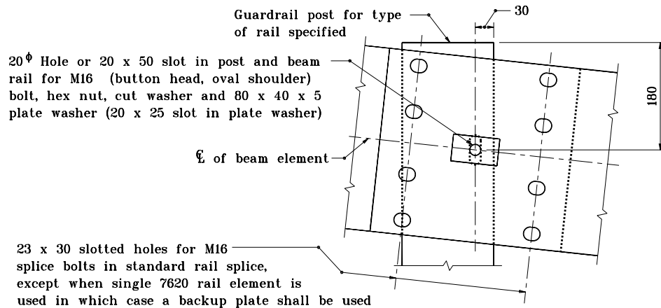
POST NO. 2 CONNECTION DETAIL
