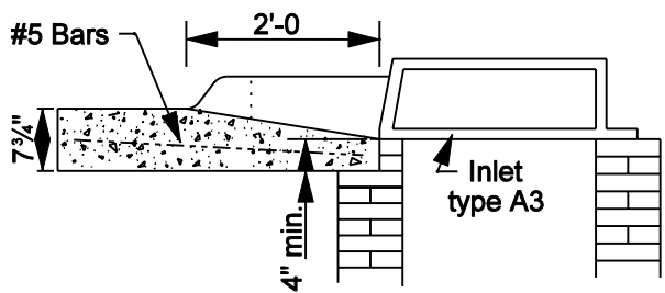
SECTION H-H
