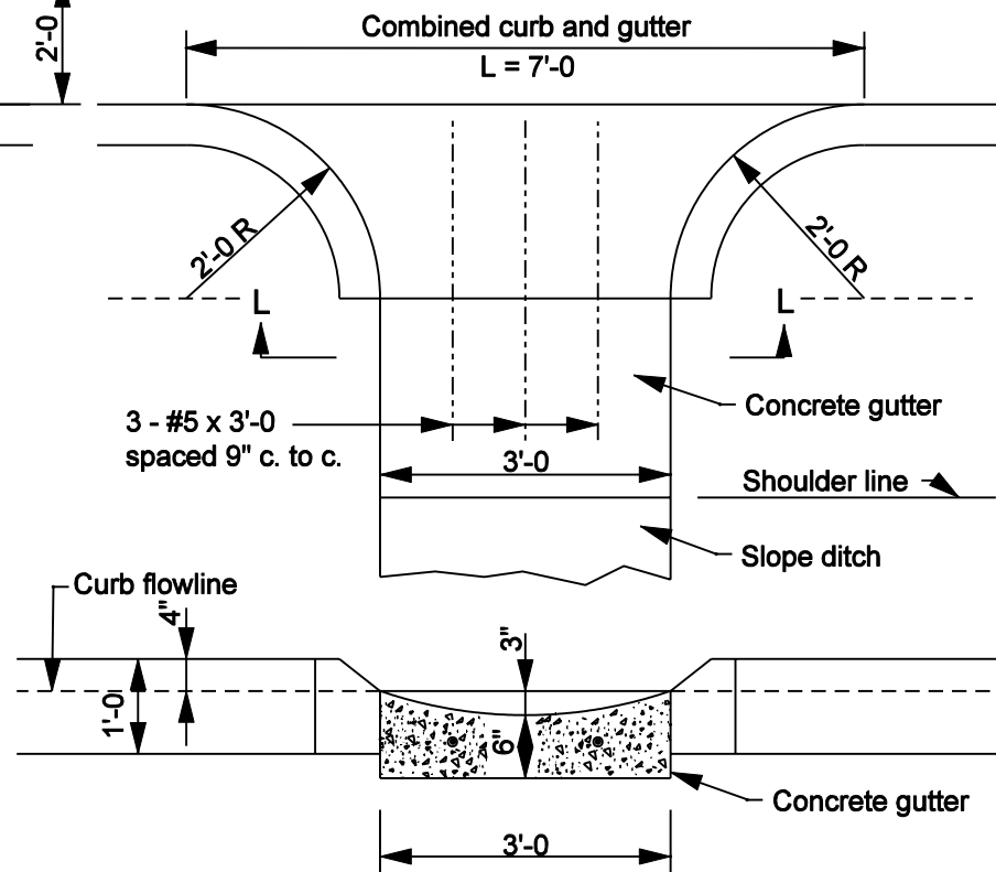
SECTION L-L
