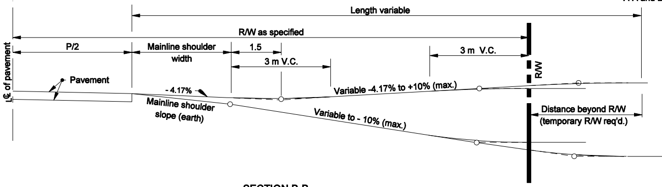
SECTION B-B APPROACH GRADE FOR CUT OR FILL TO BE USED WITH EARTH SHOULDERS
