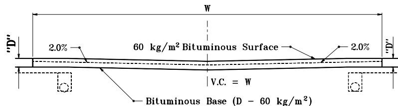
CROSS SECTION TO BE USED WITH CROWN PAVEMENTS.
