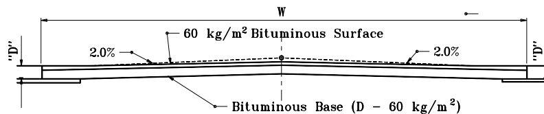
CROSS SECTION TO BE USED WITH 76 mm TILTED PAVEMENTS.
