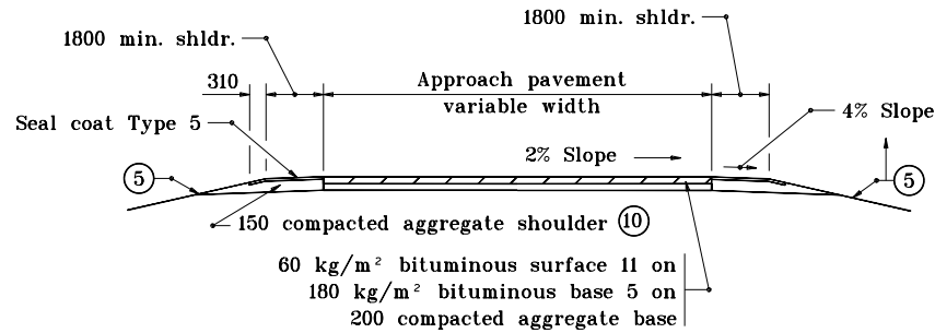
MINIMUM PAVEMENT SECTION FOR ADT THROUGH 1000
