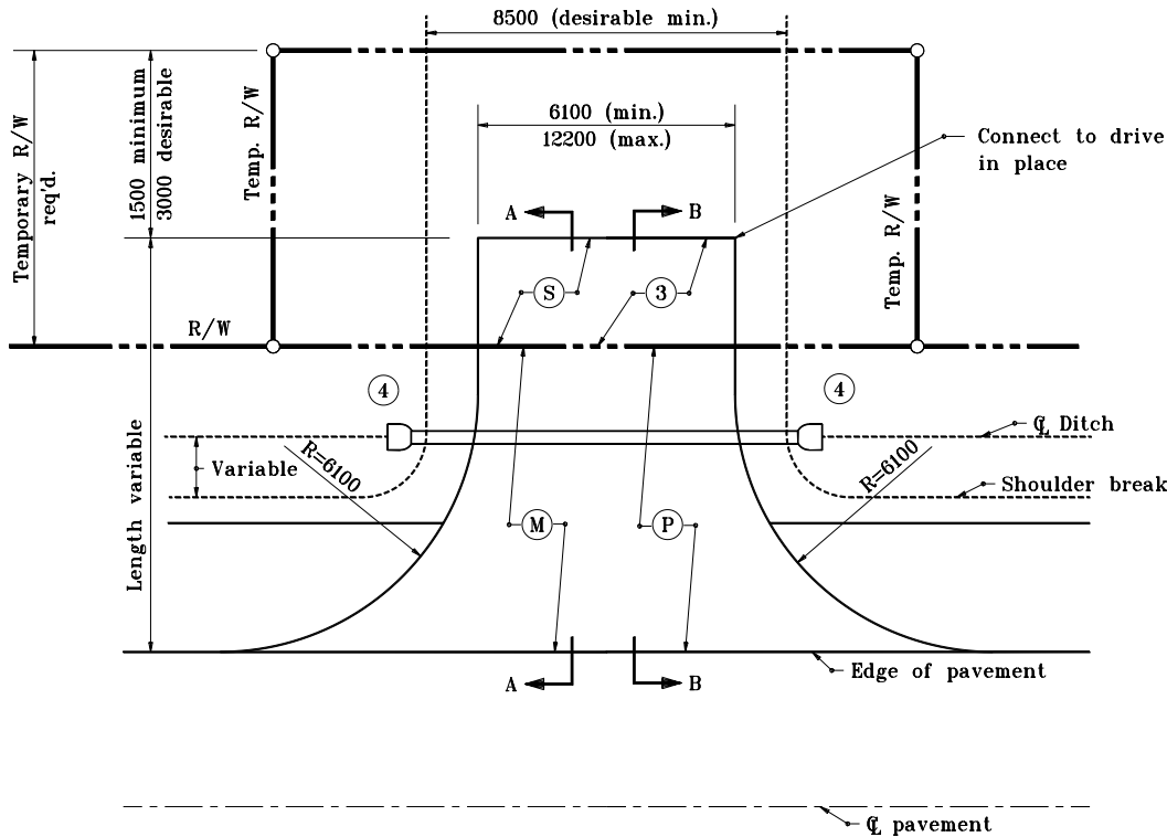
PLAN VIEW
