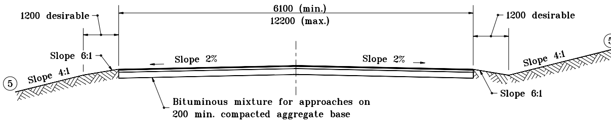
CROSS SECTION
