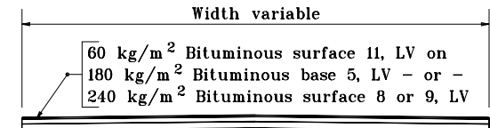
BITUMINOUS MIXTURE FOR APPROACHES TYPICAL SECTION
