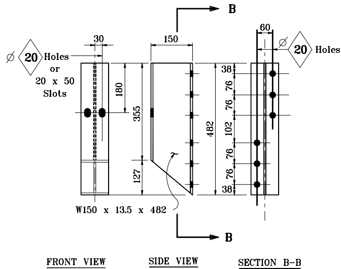
BLOCK DETAIL
