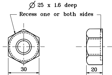
M16 RECESS NUT
