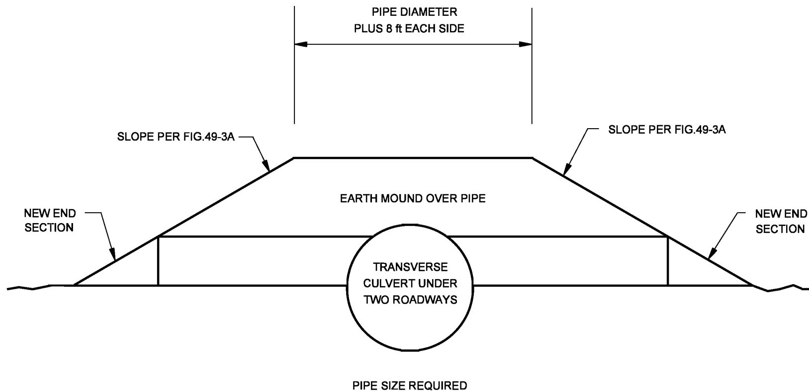
CULVERT END TREATMENT, MEDIAN SECTION
