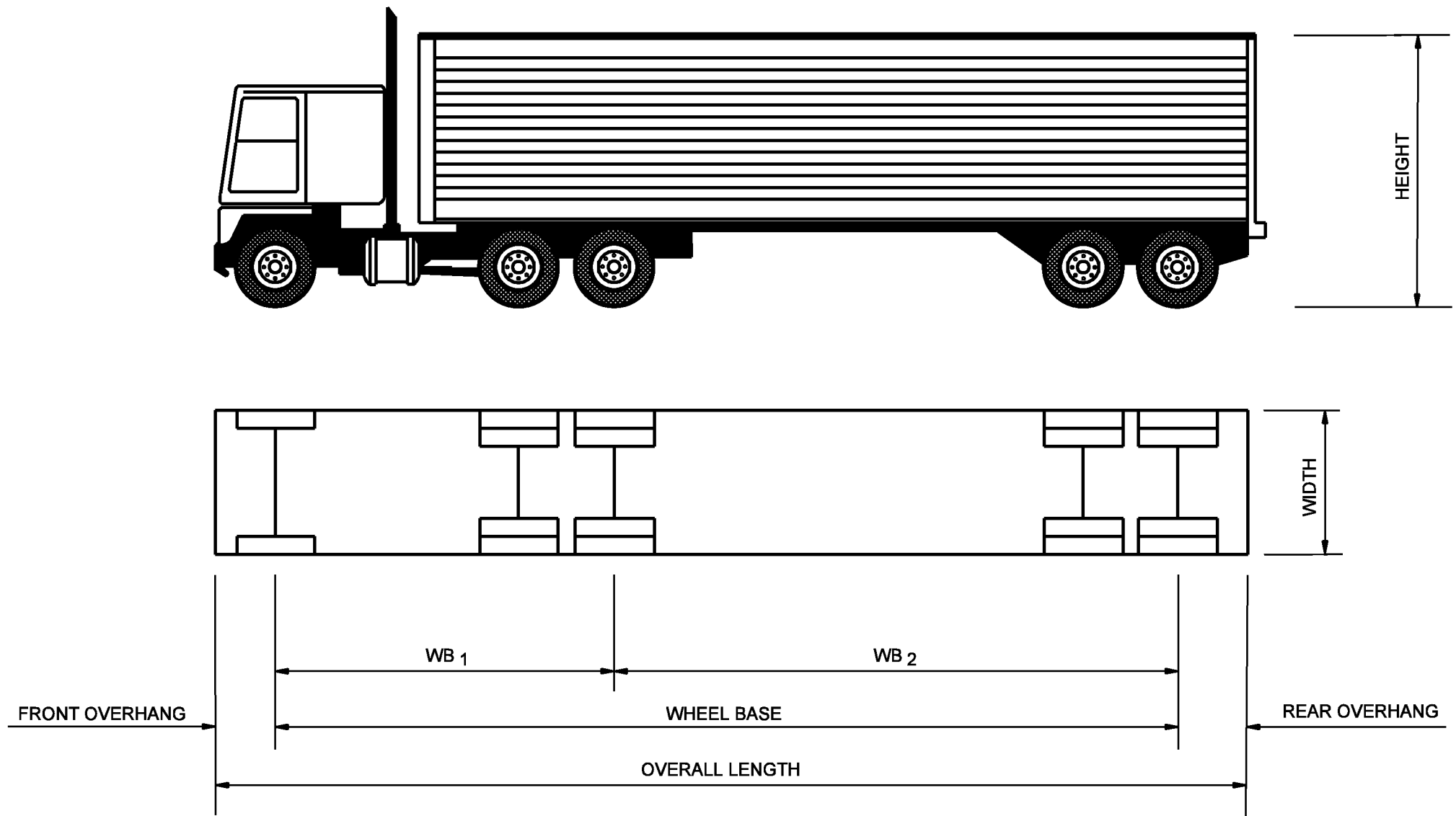
BASIC DIMENSIONS OF DESIGN VEHICLE (Combination Truck A)
