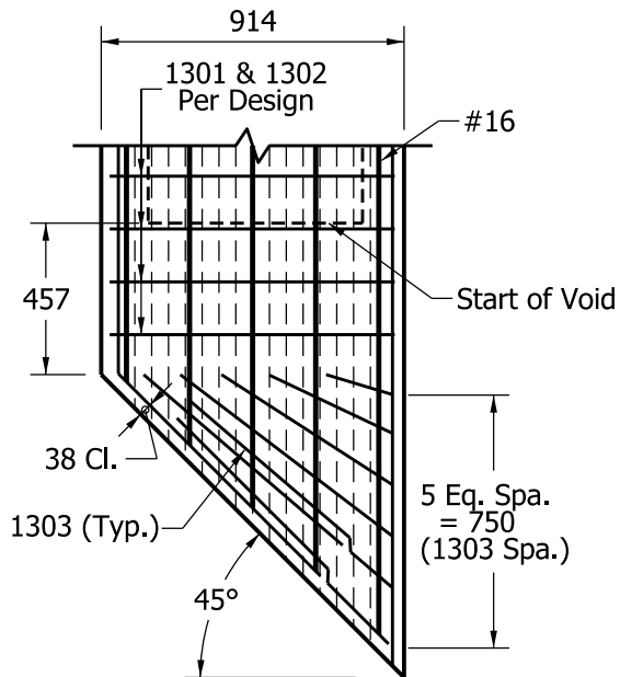
TYPICAL END REINFORCEMENT PLAN
