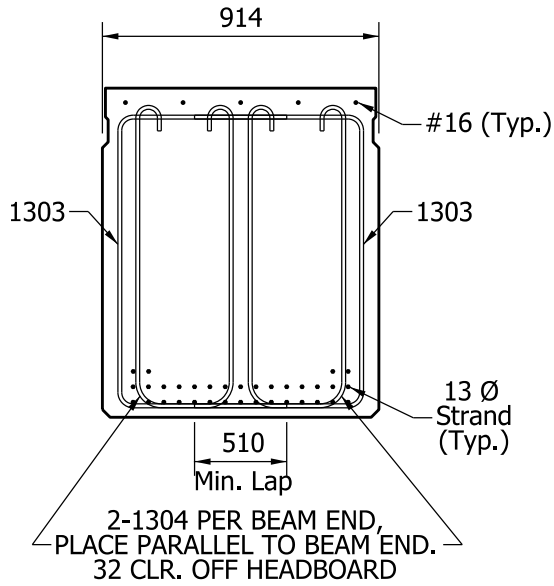
TYPICAL END REINFORCEMENT SECTION
