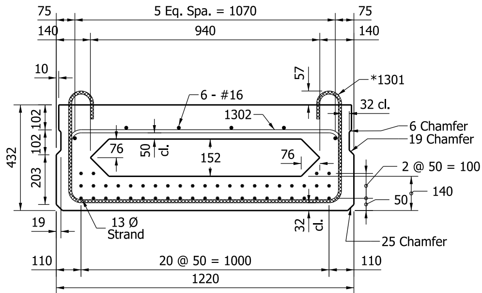
BOX BEAM TYPE CB 432 x 1220
