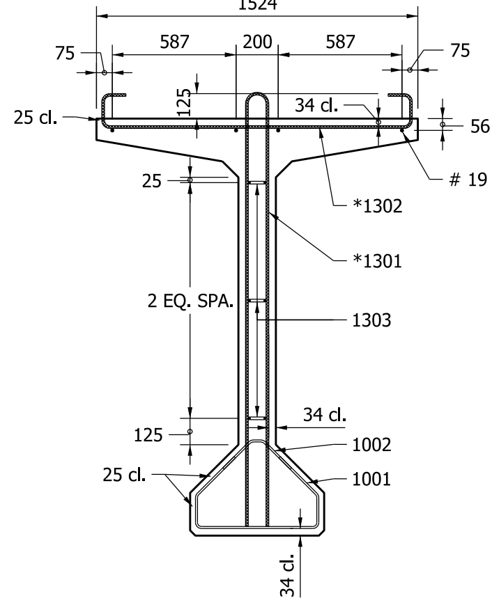
BULB - TEE BEAM TYPE BT 1981 x 1524
