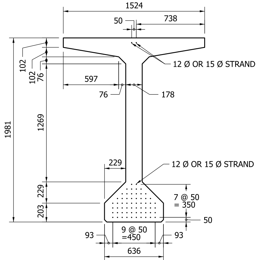
BULB - TEE BEAM TYPE BT 1981 x 1524
