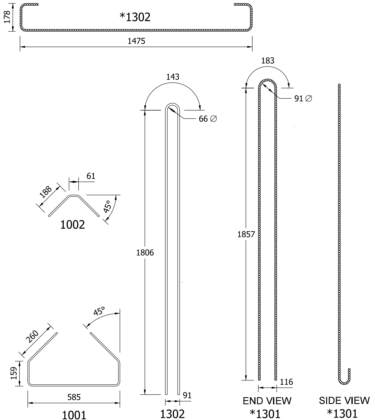
BULB - TEE BEAM TYPE BT 1829 x 1524 BAR BENDING DETAILS
