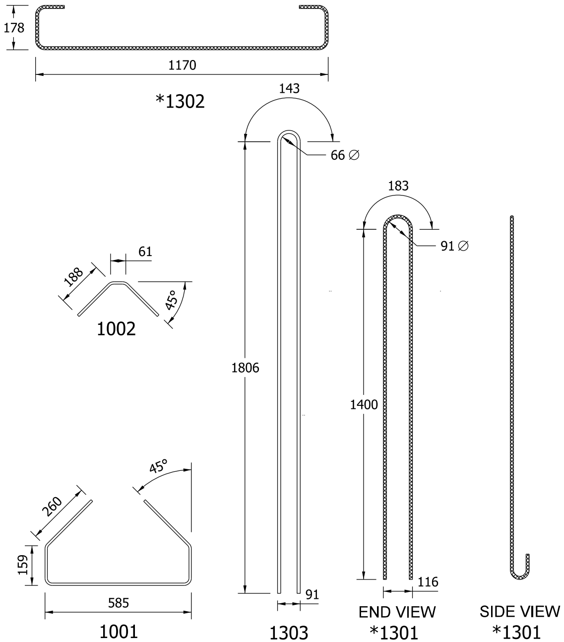
BULB - TEE BEAM TYPE BT 1372 x 1220 BAR BENDING DETAILS
