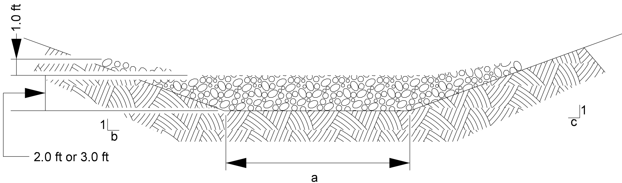
CROSS SECTION FOR DETERMINING MASS OF REVETMENT RIPRAP CHECK DAM
