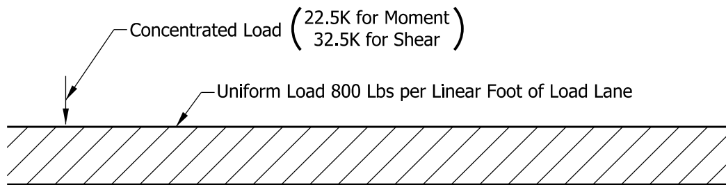
LANE HS-25 LOADINGS
