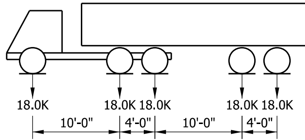
TOLL ROAD LOADING NO.1 (W = 90.0K)
