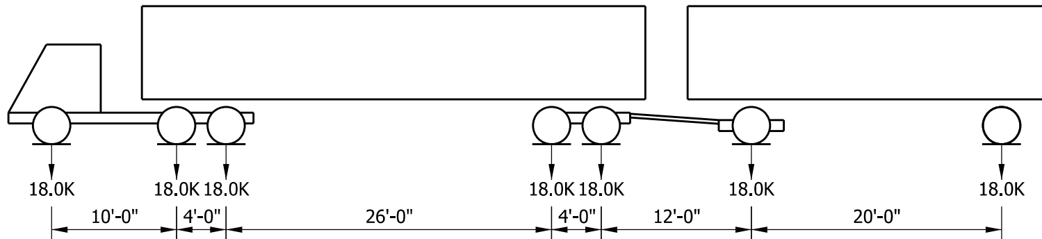
SPECIAL TOLL ROAD TRUCK (W = 126.0K)
