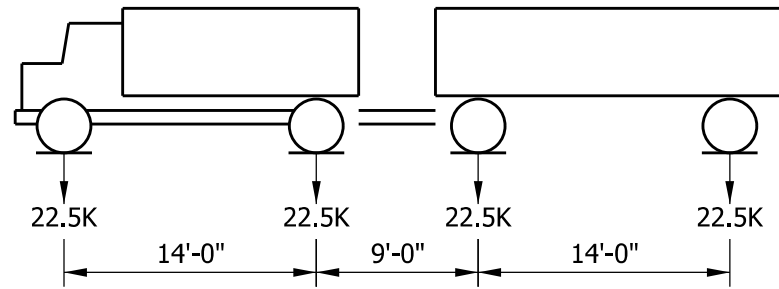
TOLL ROAD LOADING NO.2 (W = 90.0K)
