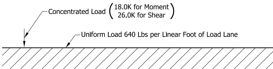
LANE H-20 LOADINGS
