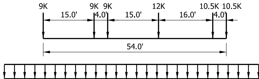
Lane Type Loading for Spans Greater Than 200 ft
