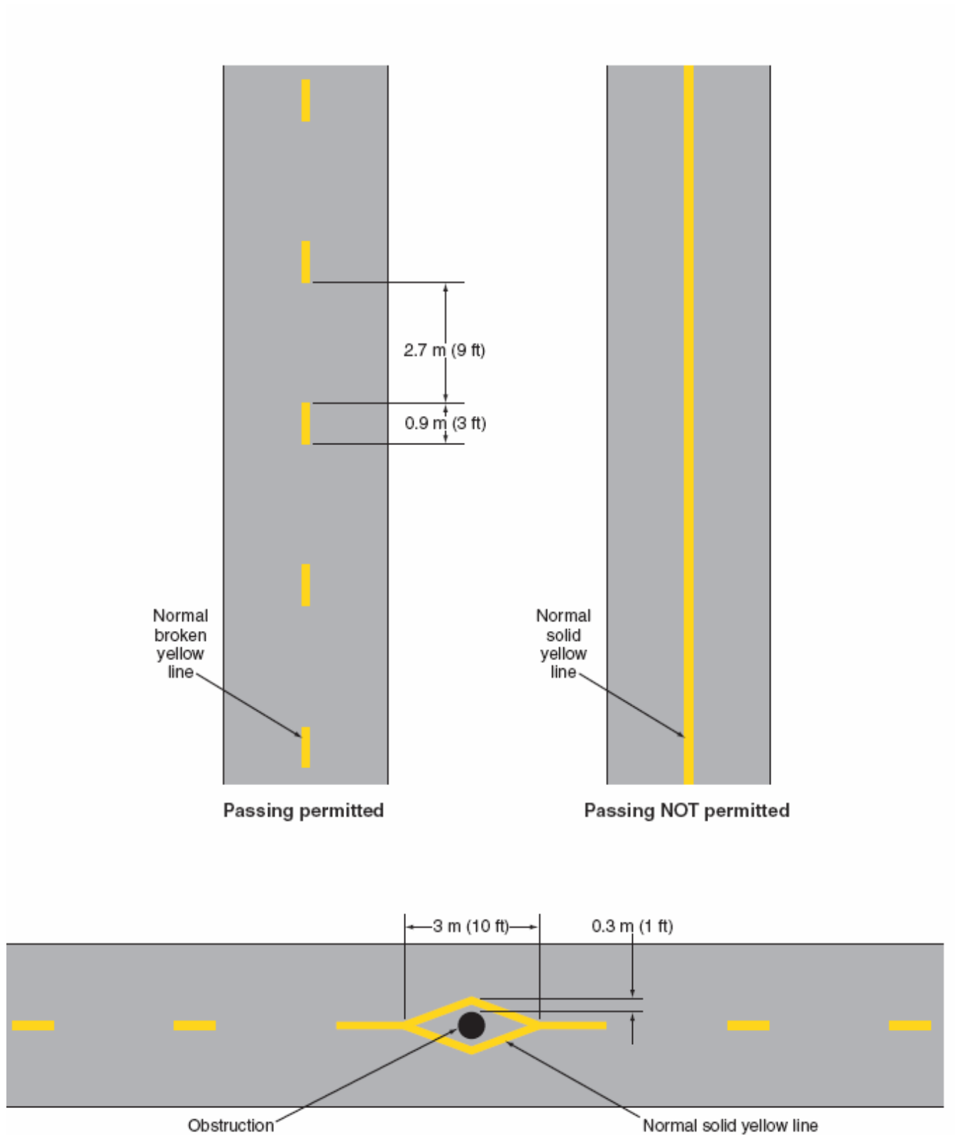
Figure 9C-2. Examples of Centerline Markings for Shared-Use Paths
