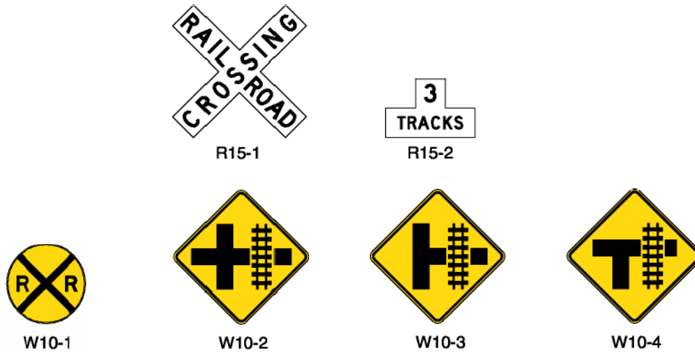
Figure 5F-1. Highway-Rail Grade Crossing Signs for Low-Volume Roads
