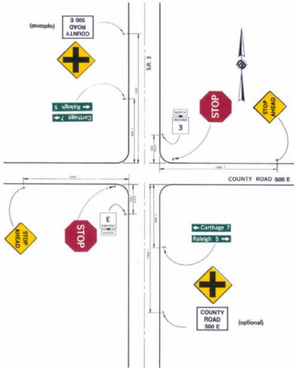
Figure 2D-6A. Illustration of Indiana Directional Assemblies and Other Route Signs Typical route markings at intersections with an Important County Road (Sheet 2 of 5)
