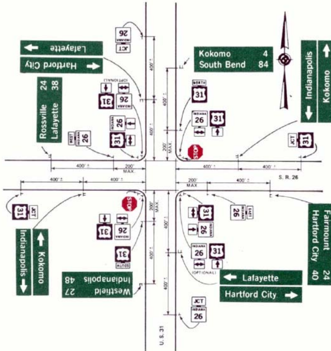
Figure 2D-6A. Illustration of Indiana Directional Assemblies and Other Route Signs Typical route markings at intersections – rural (Sheet 1 of 5)
