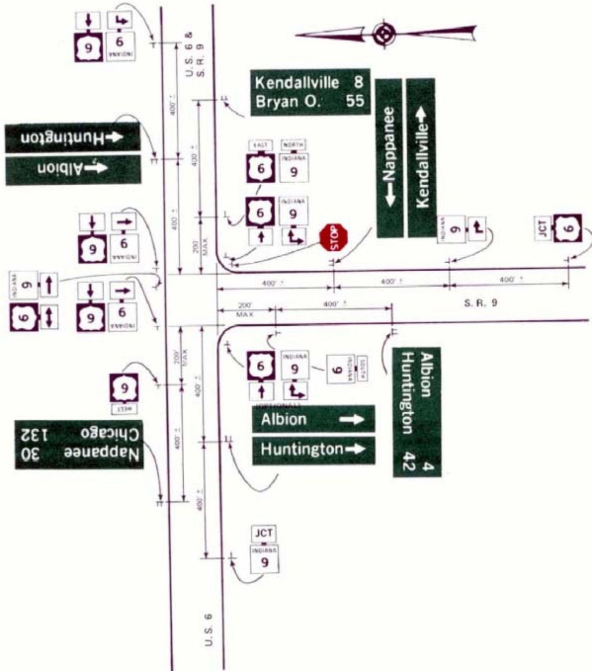
Figure 2D-6A. Illustration of Indiana Directional Assemblies and Other Route Signs Typical route markings at “T” intersections (two numbered routes – one turning) (Sheet 3 of 5)
