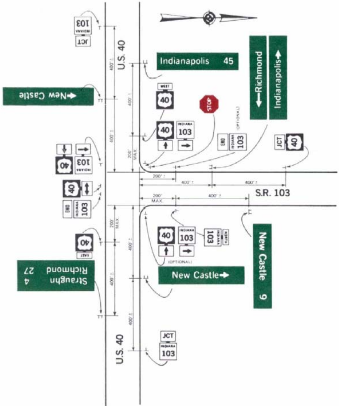
Figure 2D-6A. Illustration of Indiana Directional Assemblies and Other Route Signs Typical route markings at “T” intersections (two numbered routes – one terminating) (Sheet 4 of 5)
