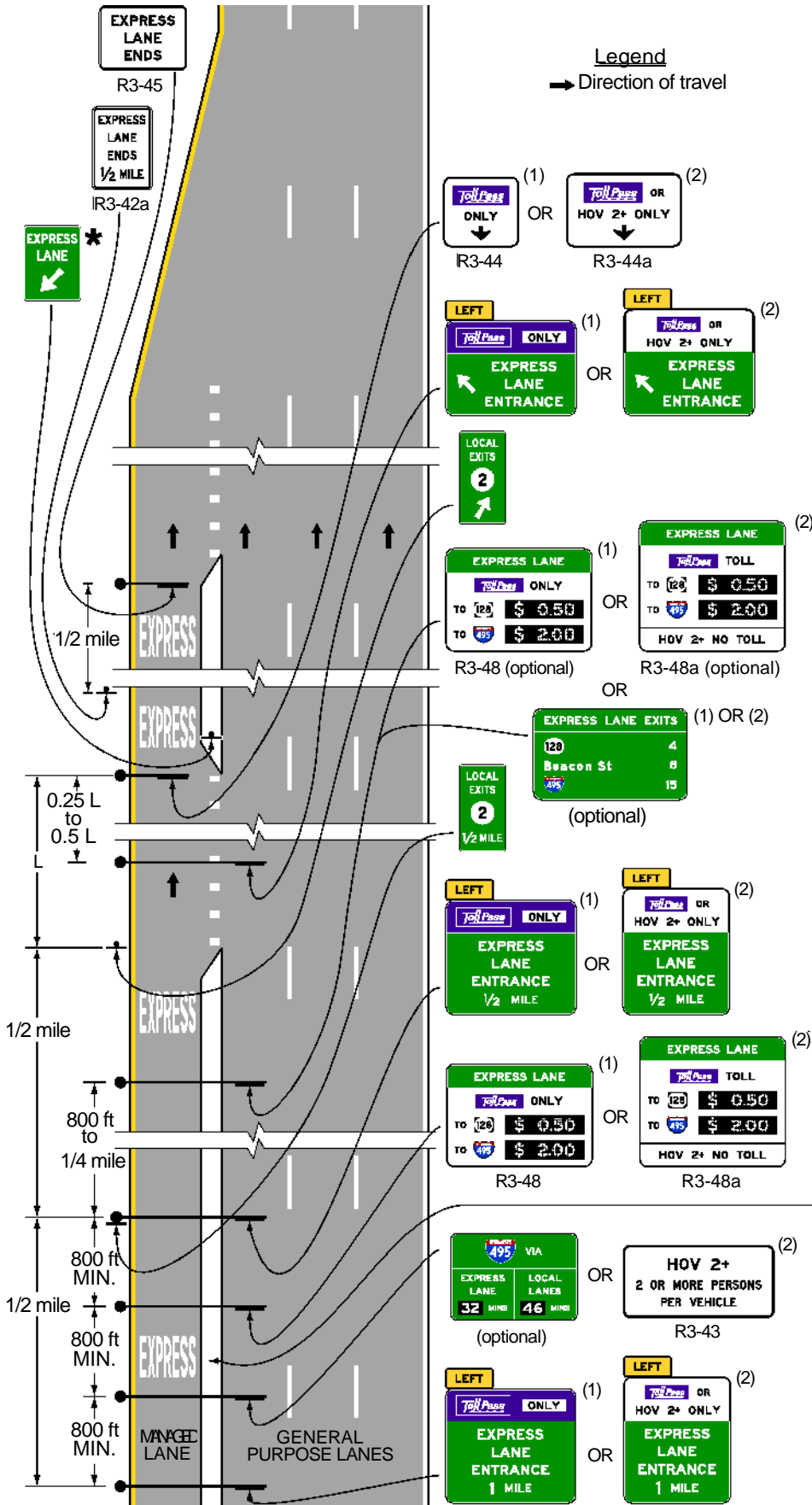
Figure 2G-24. Example of Signing for the Intermediate Entry to, Egress from, and End of Access-Restricted Priced Managed Lanes
