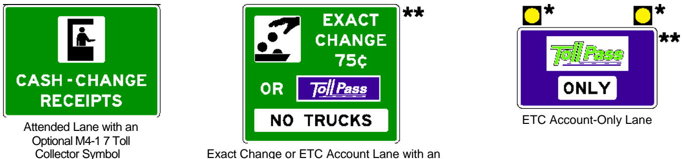
Figure 2F-9. Examples of Toll Plaza Canopy Signs
