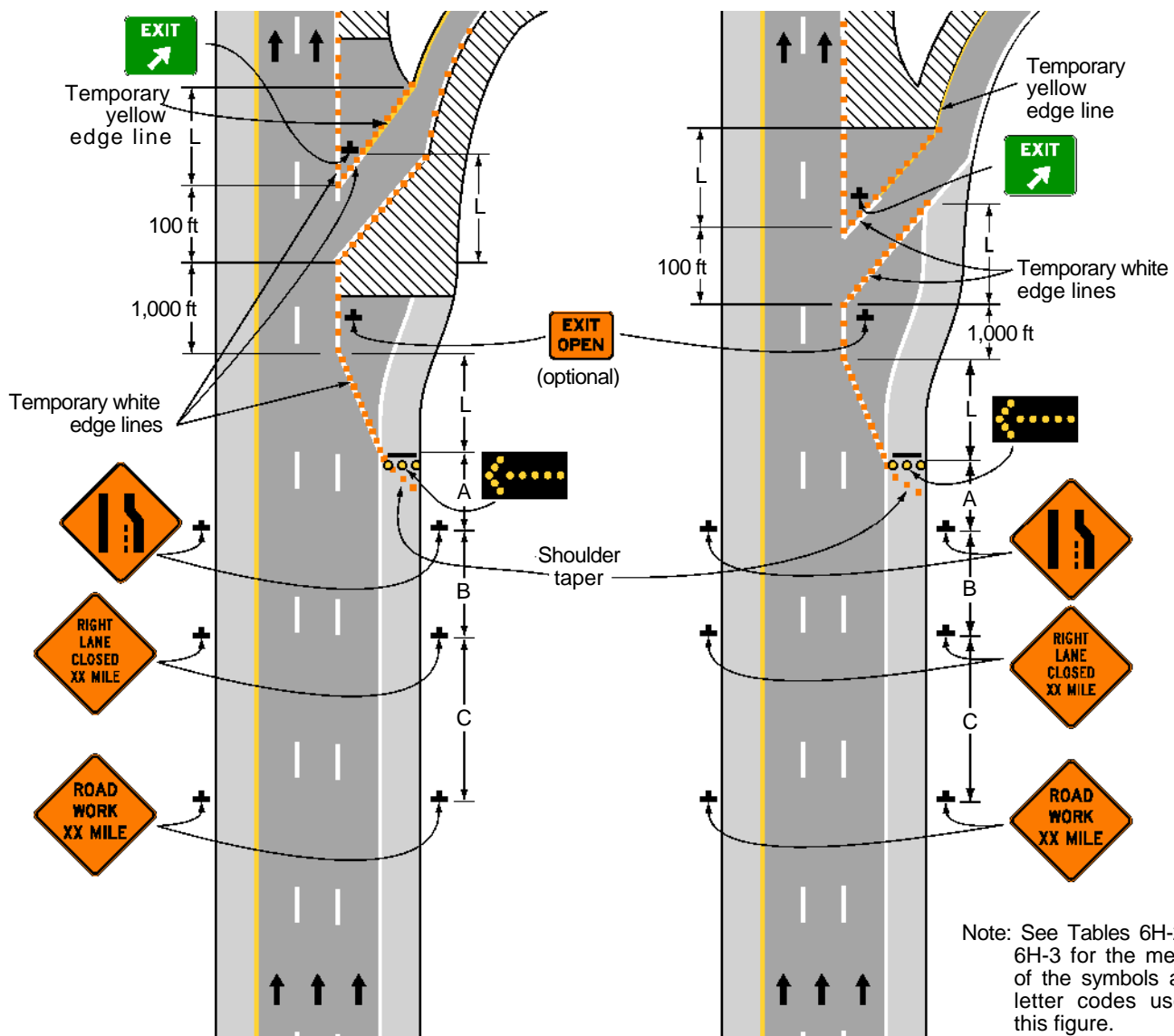
Typical Application 42
