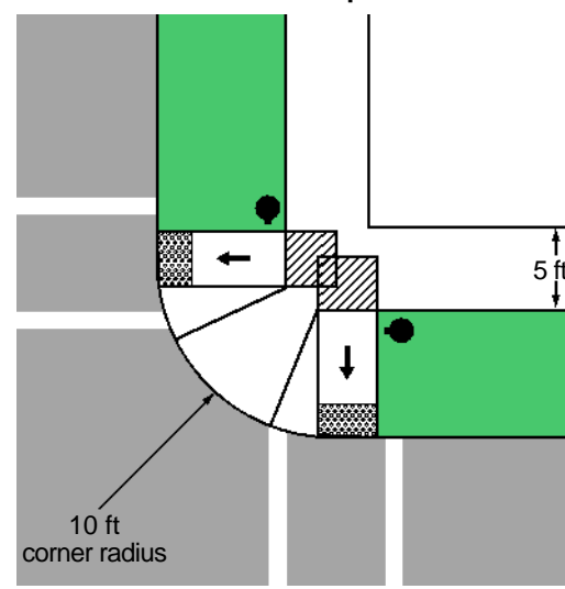
H - Perpendicular ramps with sidewalk set back from road with continuous sidewalk between ramps
