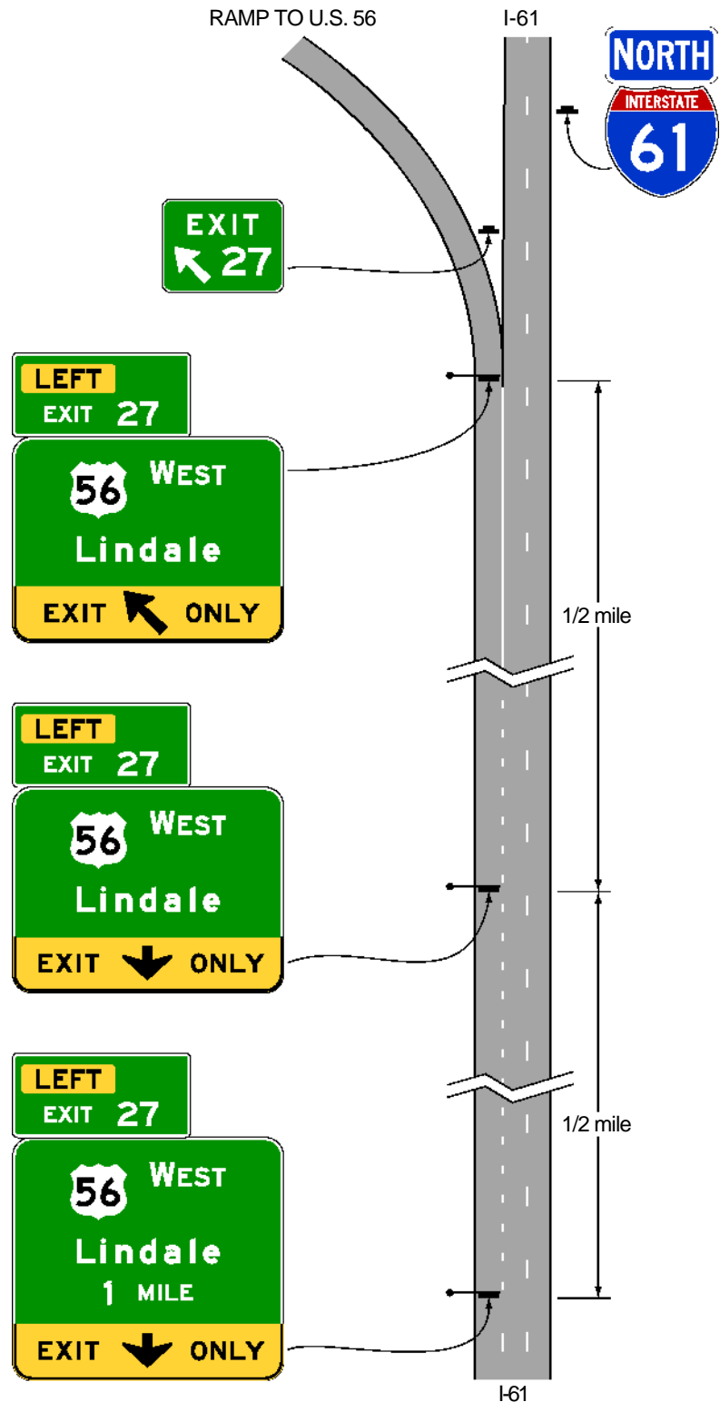
Figure 2E-15. Guide Signs for a Single-Lane Exit to the Left with a Dropped Lane
